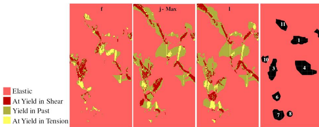
Figure 5: Occurrence of plastic deformation at the moment just prior to reaching the UCS value (left), at the peak value (middle) and just after the peak (right). The extreme right picture illustrates the position and size of the soft inclusions (in black)
