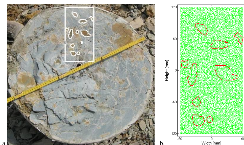
Figure 2: a. Section through a soil mix column; in this section a rectangular sample with dimensions of 120 \times 240 mm is selected; b. Mesh generated for the discontinuous simulations (red lines indicate the soil inclusions)
