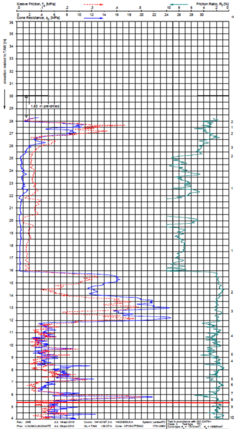
Figure 18. typical CPTe at the job site in the Mons area
