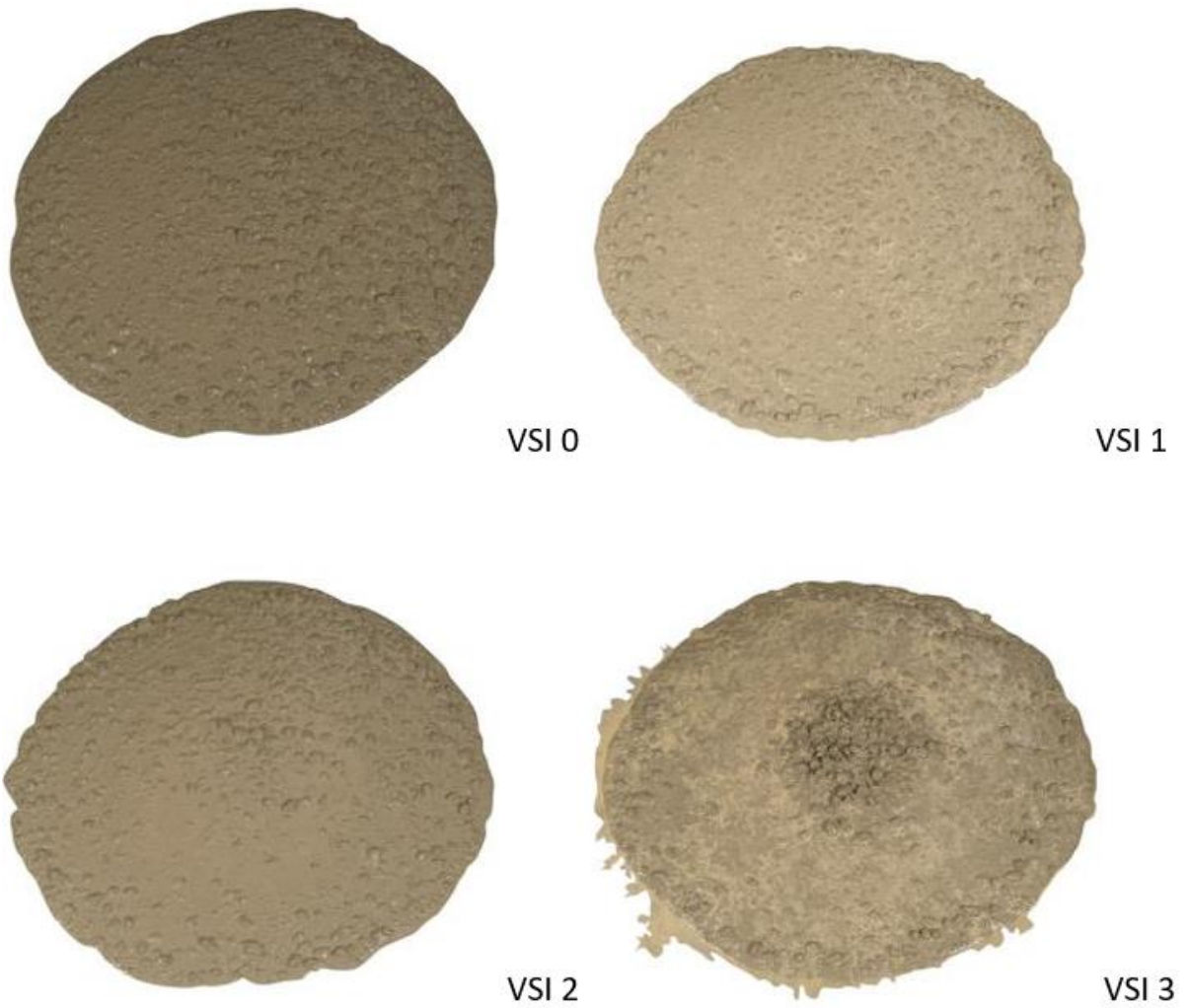
Figure 29. Examples of Visual Stability Index Classes [1], photo courtesy of BASF Corporation
