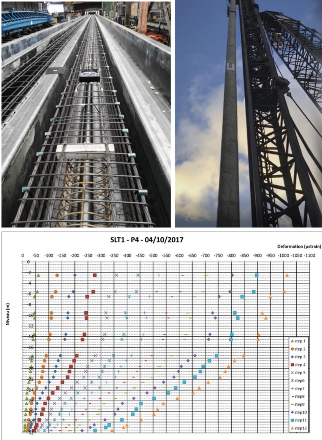
Figure 36. Instrumentation and compressive load tests on precast driven piles (part of Rotterdam)
