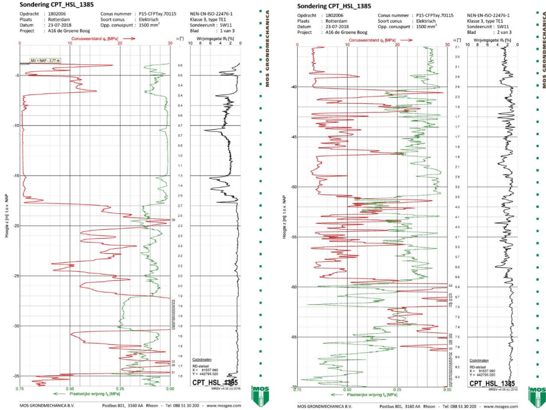
Figure 21. typical CPTe results on the site
