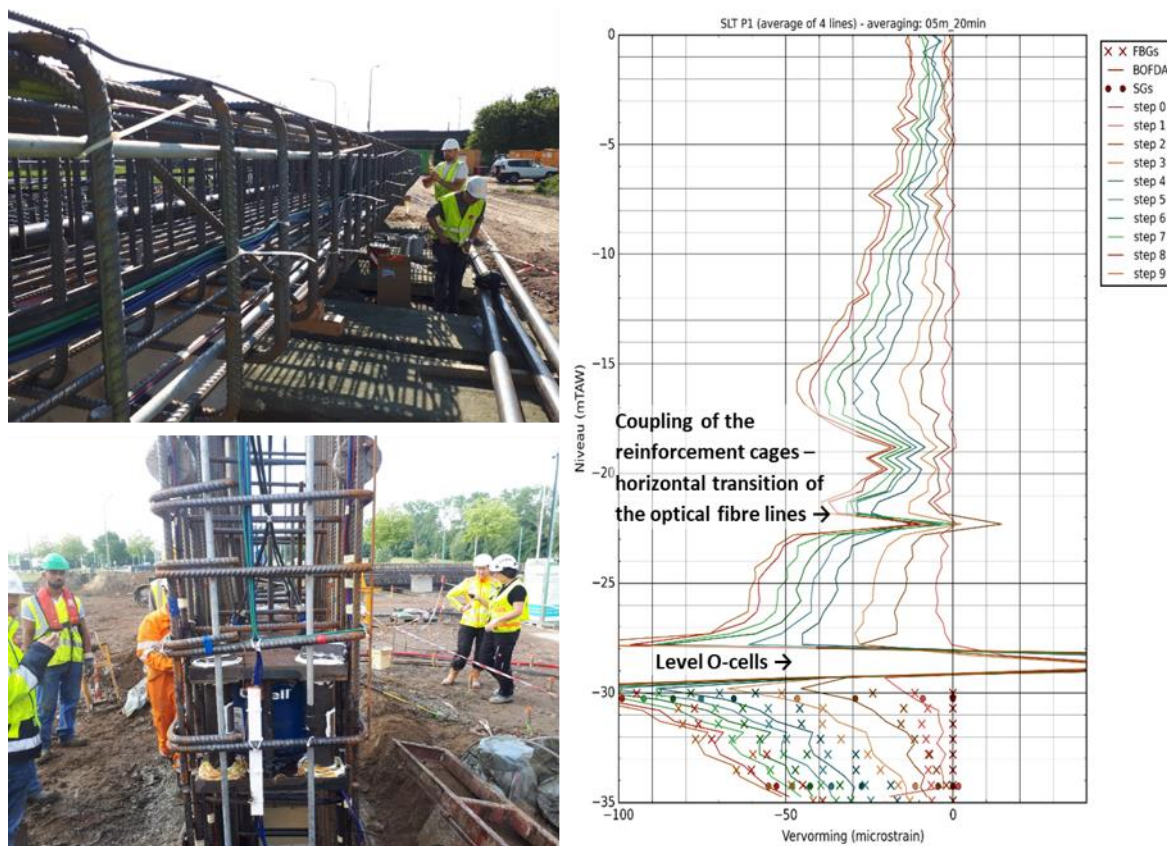
Figure 37. Instrumentation and O-cell load tests on diaphragm walls in Antwerp (Lantis)
