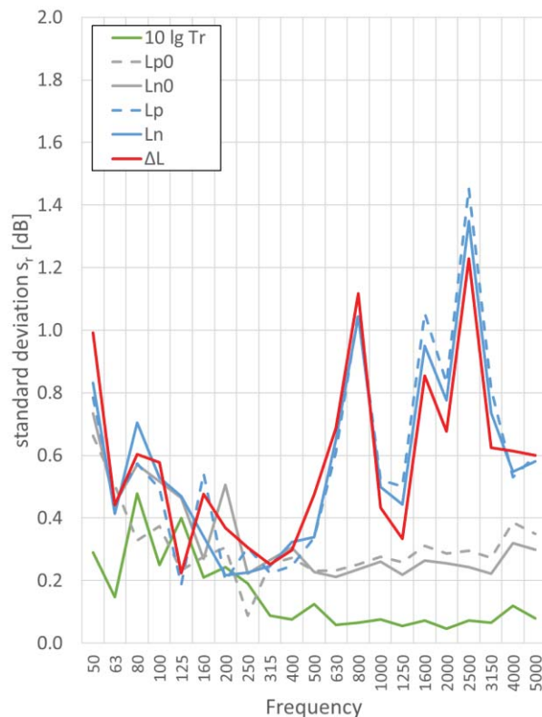
Figure 5 –Standard deviation under repeatability conditions for the different measurands determining \Delta L
