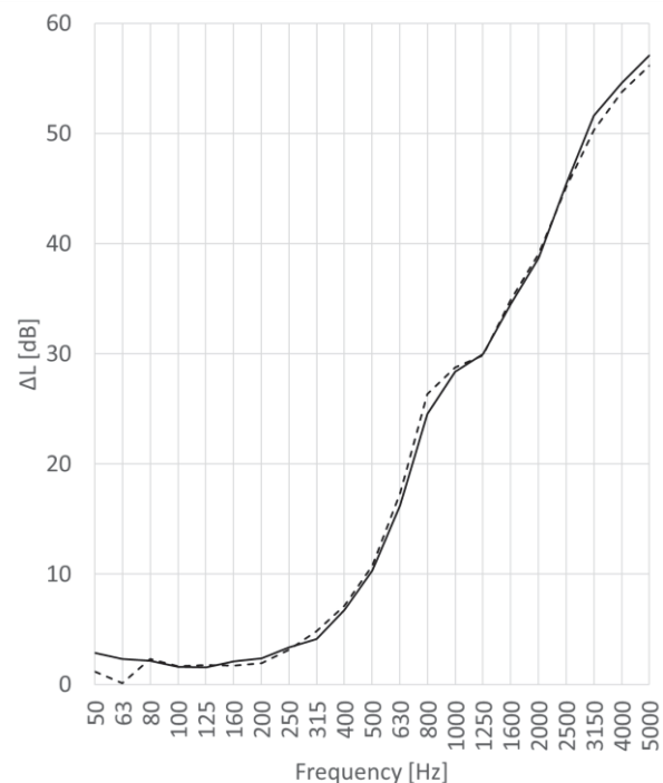
(b) Influence of the bare floor edge conditions on \Delta L
