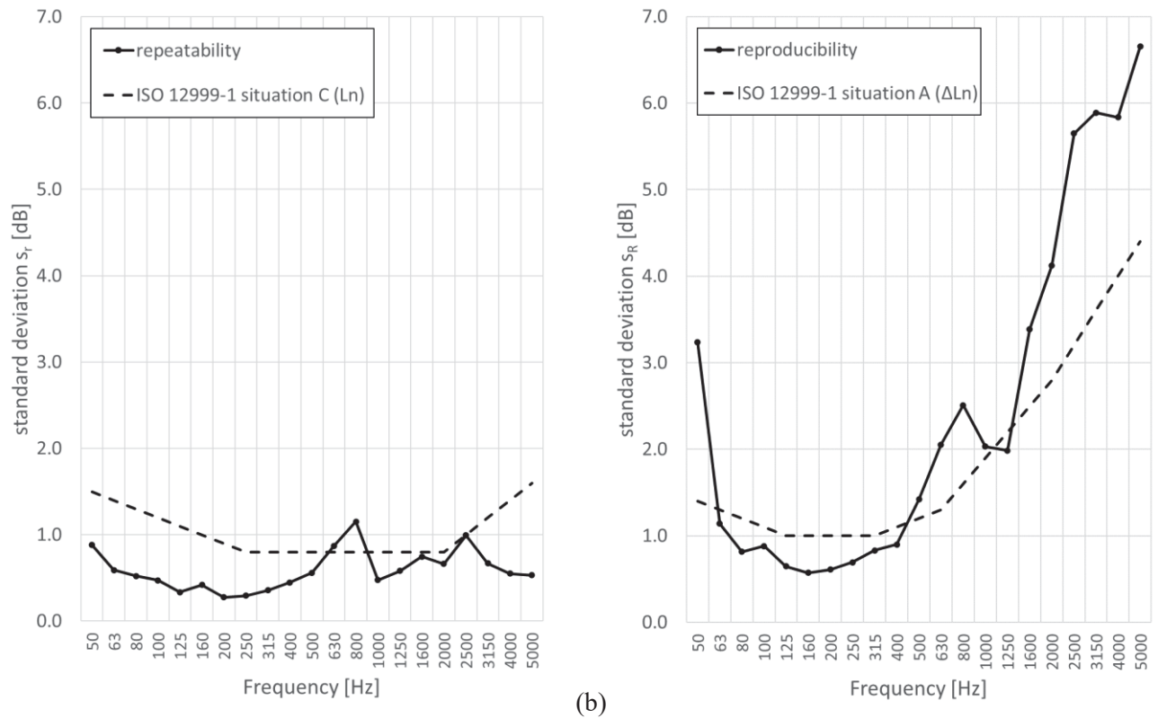
Figure 4 – Standard deviation under (a) repeatability and (b) reproducibility conditions for \Delta L of the vinyl floor covering.
