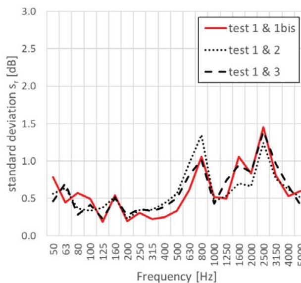
Figure 7 – Standard deviation for L_p under repeatability conditions for the same sample (test 1 & 1bis) or different samples (test 1 & 2 and test 1 & 3).
