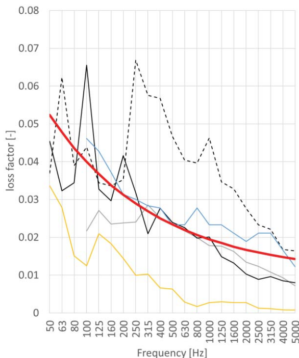
(a) Loss factor measured at 4 laboratories and minimum loss factor required by ISO 10140 (red)
